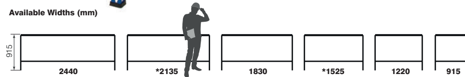
Half Undersheff Workbench with Chipboard Tops 915 x 1830 x 915
